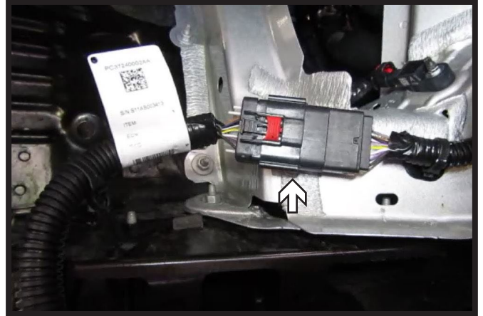
12. Unplug the electrical on the passenger side of the vehicle.
